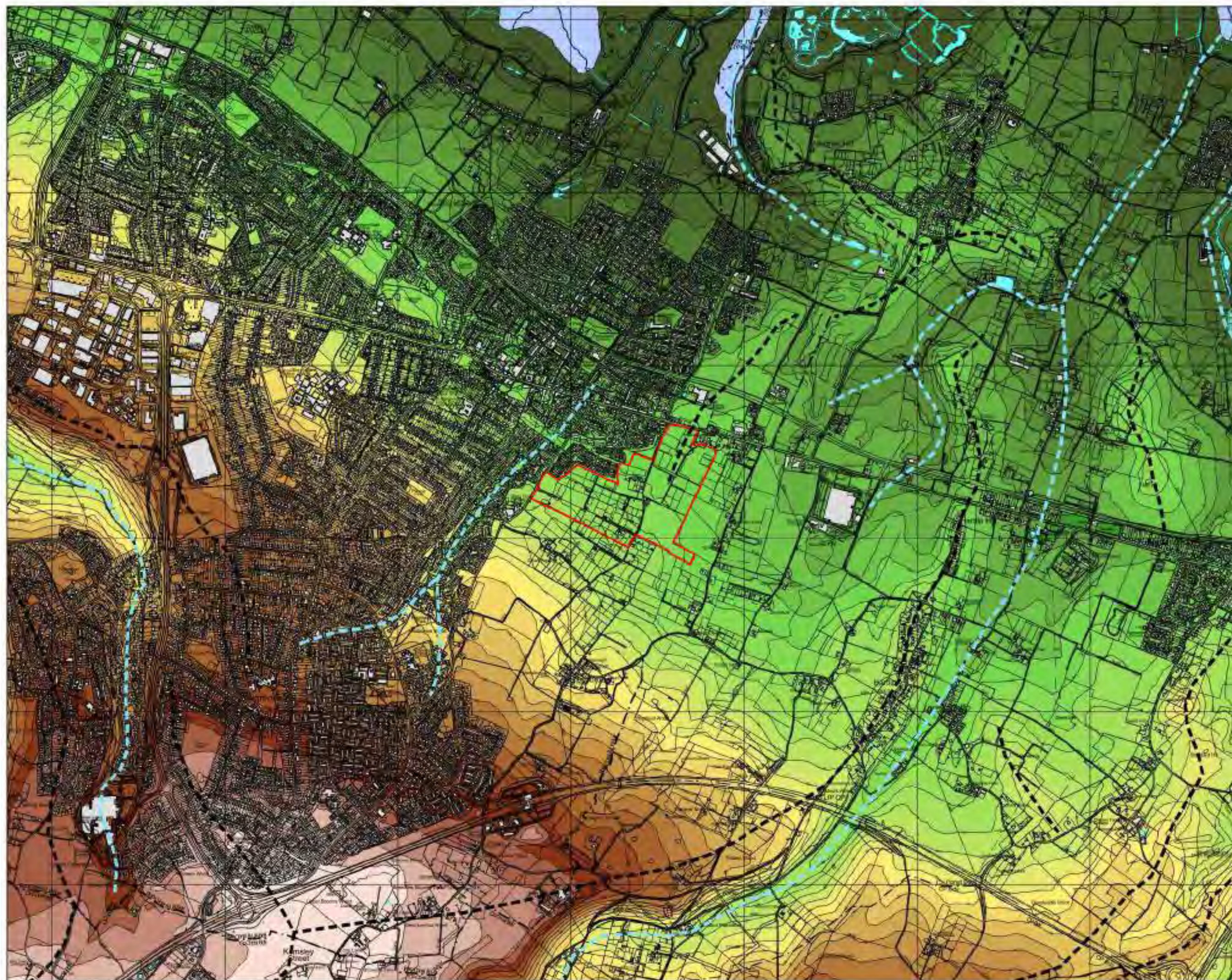
FIGURE 2 Project: Land East of Rainham Medway Drawing Title: Topography Plan
